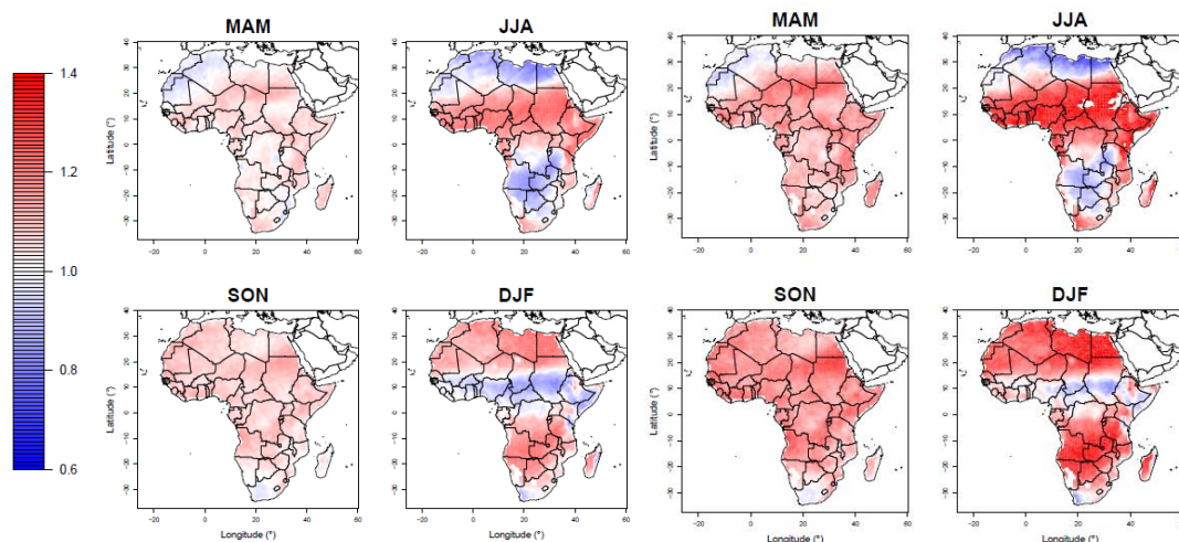
213 Figure 4: ORL95_{lat}^{sea} / ORL95_{lat}^{cst} (period 2005-2016). Amplitude of demand seasonality: 30% (left); 50% (right).
